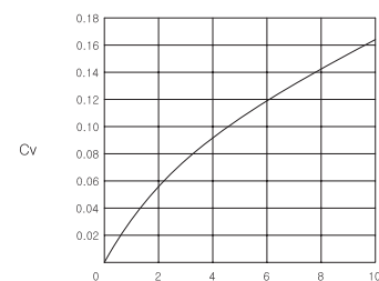
Turn Open Valve Handle SMTV3 Series
