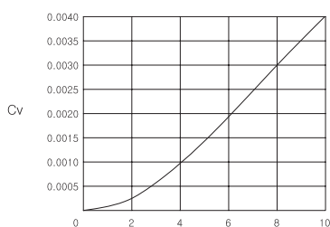
Turn Open Valve Handle SMTV1 Series
